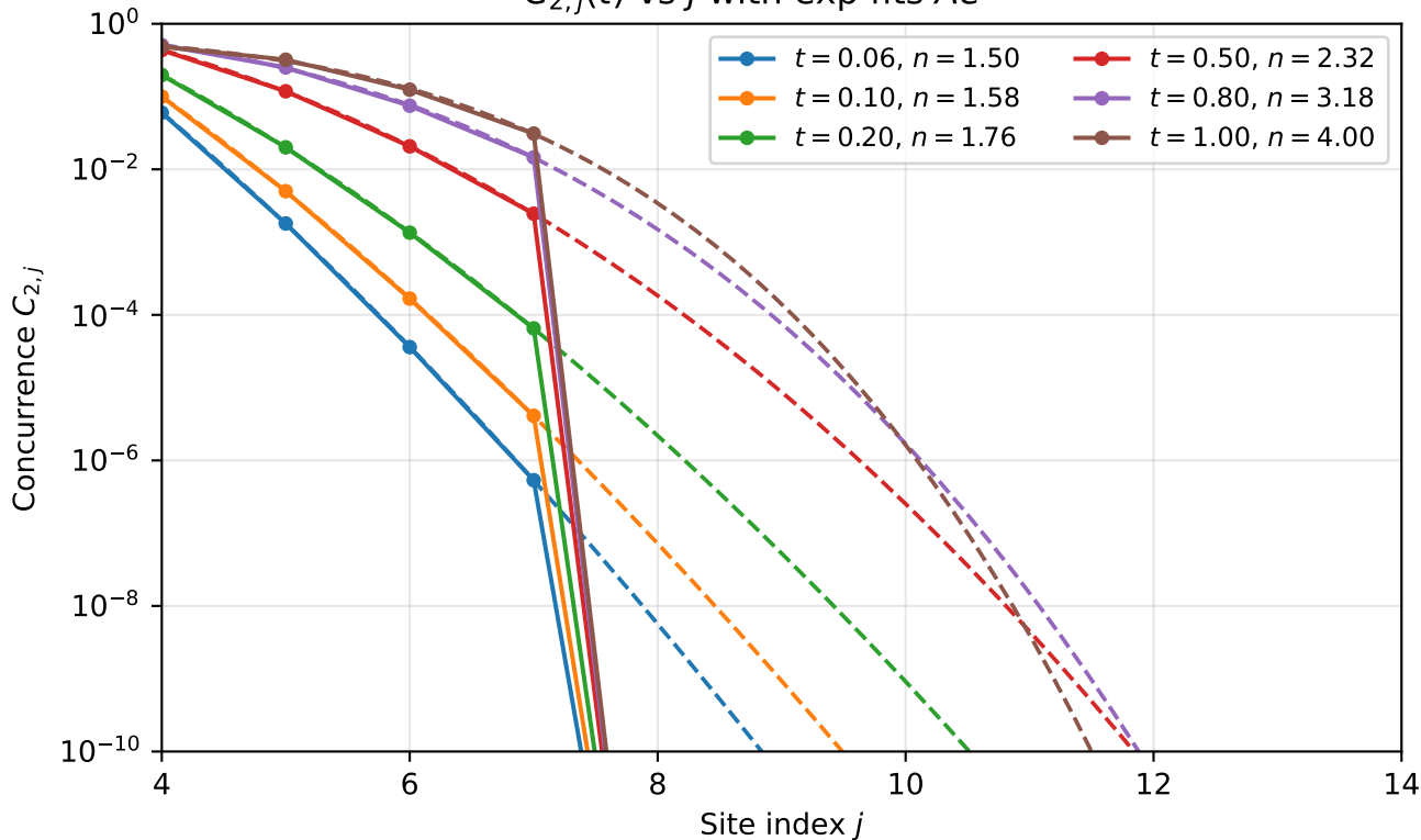
C_{2,j}(t) \text{ vs } j \text{ with exp fits } Ae^{-kj^n}
